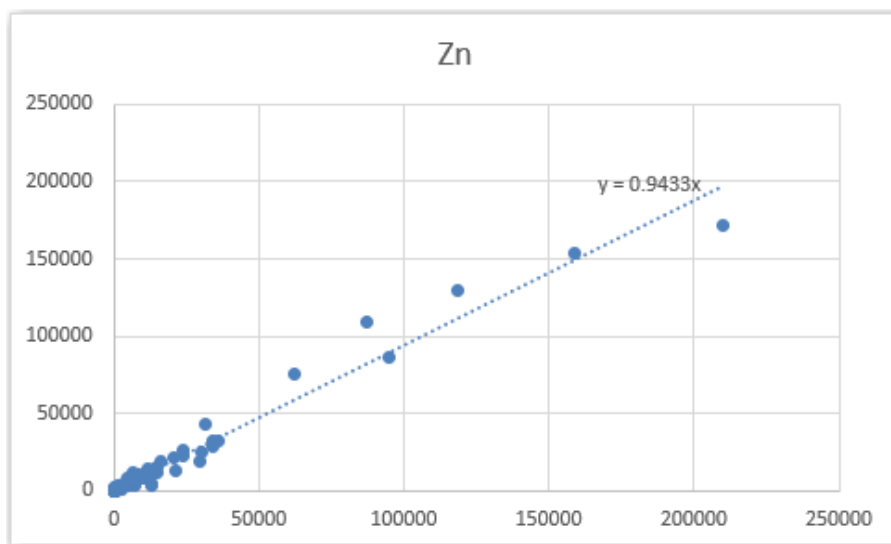
FIGURE 11-5: FIELD DUPLICATE RESULTS – Zn
