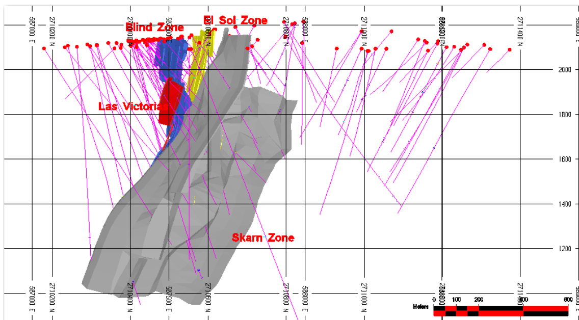
FIGURE 14-3: SECTION VIEW OF CERRO LAS MINITAS MINERALIZED ZONES AND DRILL HOLES LOOKING 325 DEGREES AZIMUTH
