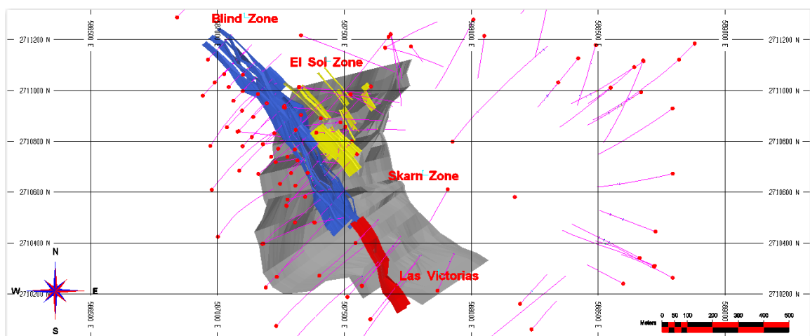
FIGURE 14-2: PLAN VIEW OF CERRO LAS MINITAS MINERALIZED ZONES AND DRILL HOLES
