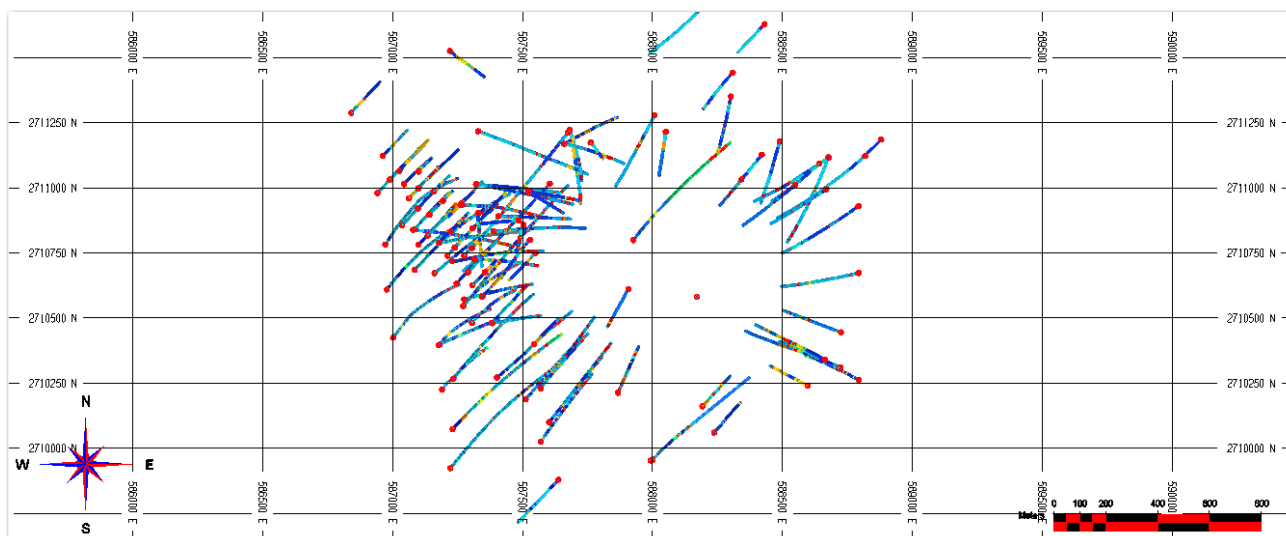
FIGURE 14-1: PLAN VIEW OF CERRO LAS MINITAS DRILL HOLES
